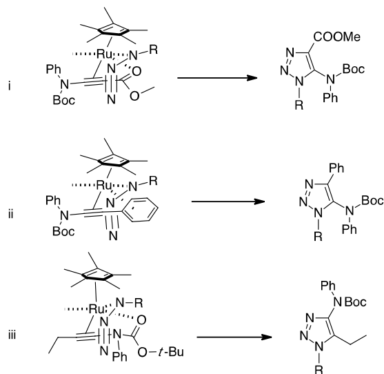
SCHEME 4. Proposed intermediates for the different regiochemical outcome: i and ii justify the selectivity toward the 5-amino substituted triazole, iii justifies the formation of the 4-amino substituted triazole in the reaction with alkyl N-Boc-ynamides.
