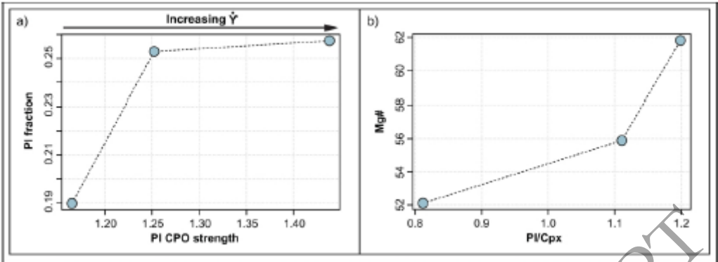
1528 Fig. 12 – a) Pl CPO strength versus Pl fraction; b) Residual glass Mg# variation as a function of Pl/Cpx 1529 fraction variation.
