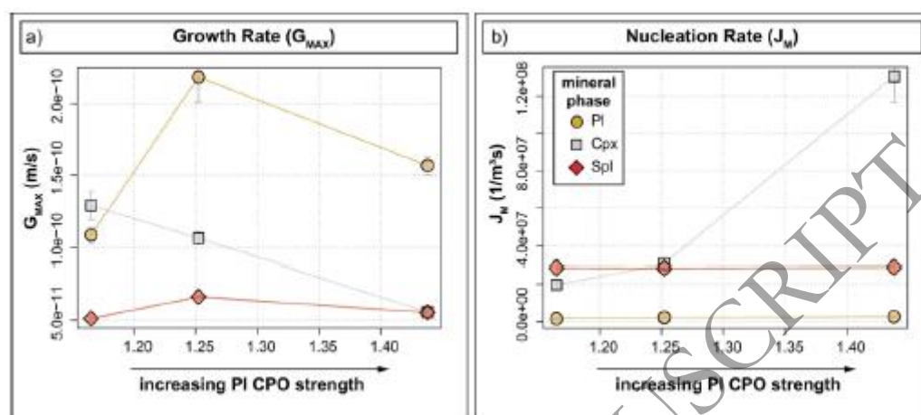
Fig. 11 – a) Pl, Cpx and Fe-Spl growth rates ( G in m/s) plotted against the CPO strength. b) Pl, Cpx and Fe-Spl nucleation rates ( J in 1/\text{m}^3\text{s} ) plotted against the CPO strength. Error bars on G_{\text{MAX}} represent the standard error for G_{\text{MAX}} calculated from the ten largest crystals in each map, reflecting the precision of the mean estimate. Error bars on J_M represents uncertainties propagated error from crystal size correction and crystal count.
