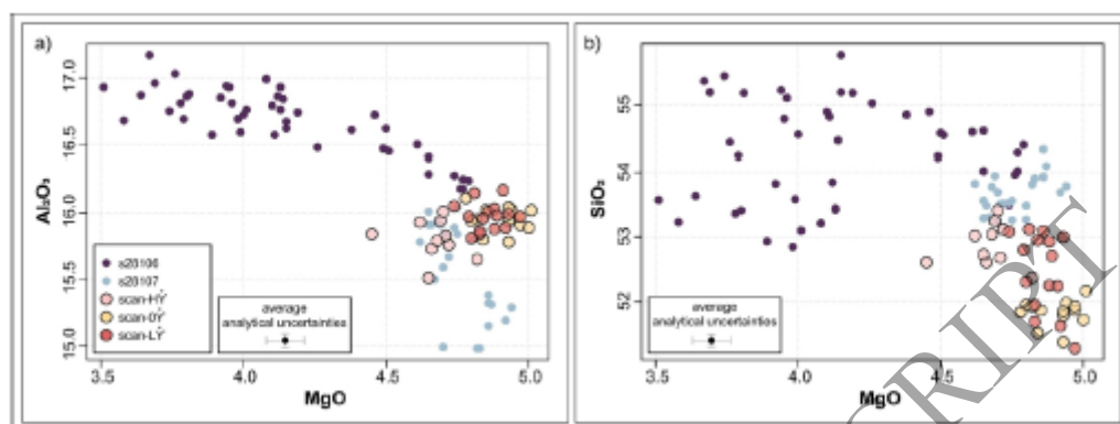
Fig. 7 – Oxide glass composition of sample Md-s28107 and Md-s28106 shown as MgO vs Al 2 O 3 (a) and MgO vs SiO 2 (b). Analytical points acquired in scans-H \checkmark , -O \checkmark and -L \checkmark have been highlighted with larger pink, yellow and red dots respectively. The MgO, Al 2 O 3 and SiO 2 average analytical uncertainties have been reported within all figures.
