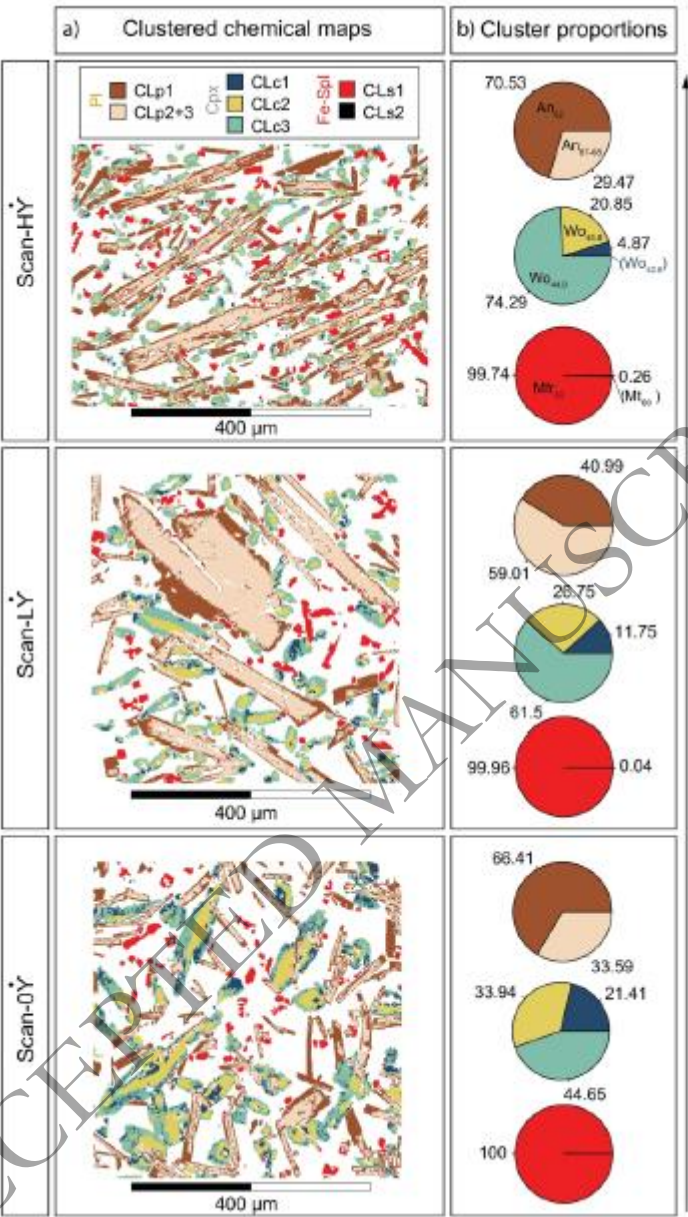
1514 Fig. 9 – a) Clustered map for each mineral phase (Cpx, Pl, Fe-Spl) in each scan area. b) cluster area 1515 proportion in each mineral phase (for each scan) expressed as area percentage.
