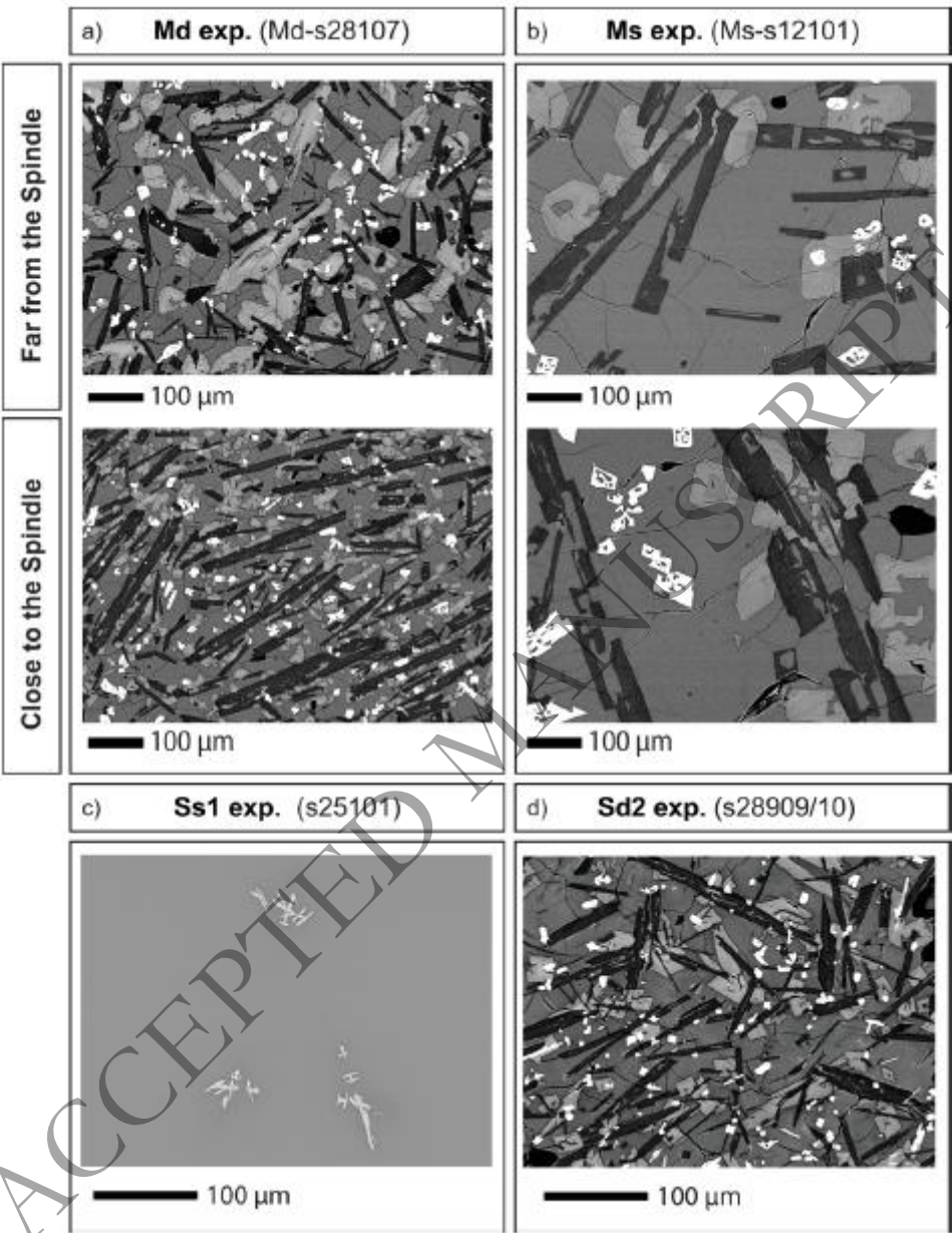
1464 Fig 2 – BSE images comparison between the static (Ms; a) and the dynamic (Md; b) main experiments, 1465 far and close to the spindle. BSE images of the static (Ss1; c) and the dynamic (Sd2; d) snapshot 1466 experiments.
