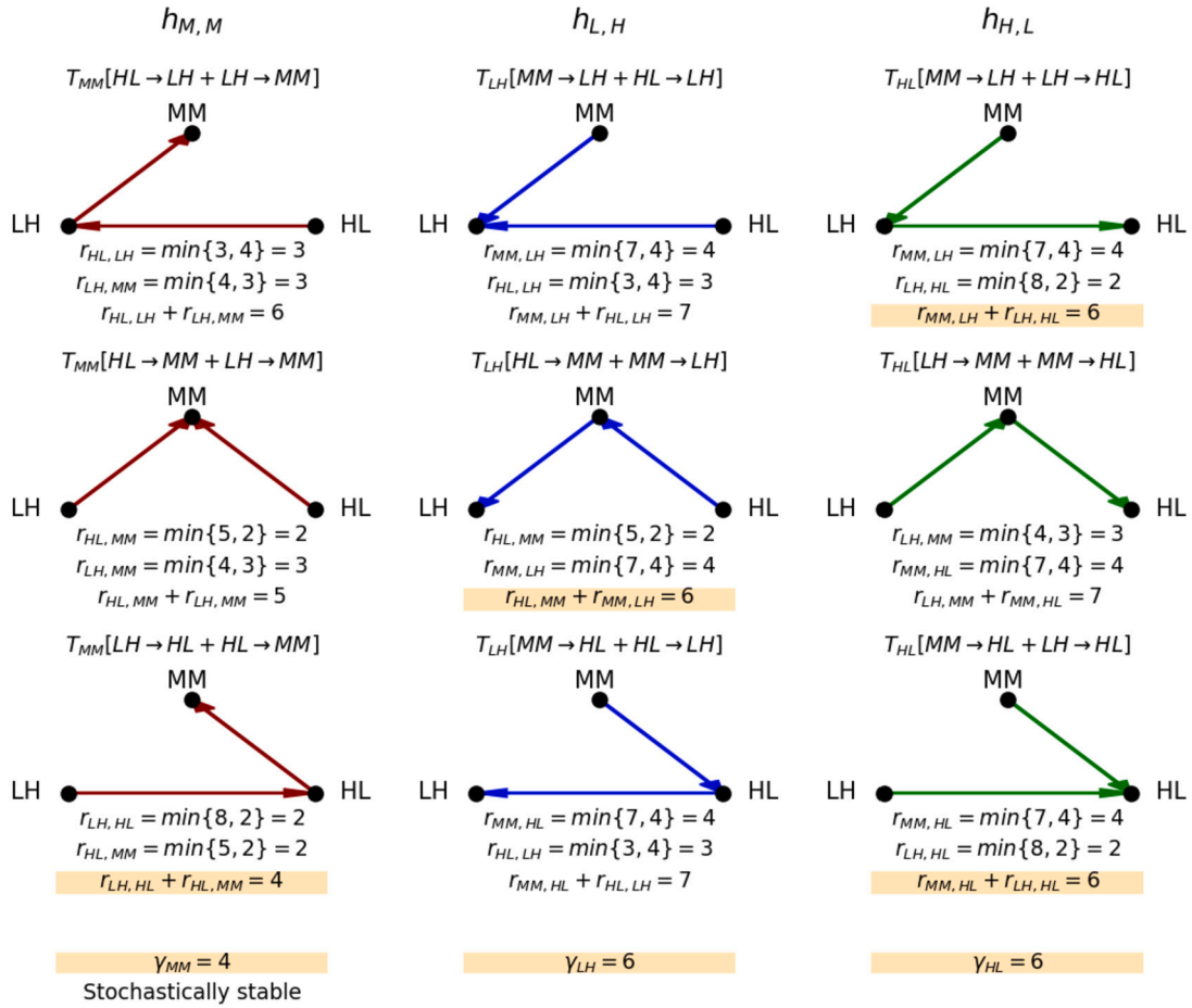
Fig. 3. Each convention has three rooted trees: on the left, the trees rooted in h_{M,M} in red; on the center, the trees rooted in h_{L,H} in blue; on the right, the trees rooted in h_{H,L} in green. Below each tree, there are indicated the resistances of the transitions of its edges, along with their sum, which represents the resistance of the tree. The stochastic potential of each convention is highlighted in yellow. (For interpretation of the colors in the figure(s), the reader is referred to the web version of this article.)
