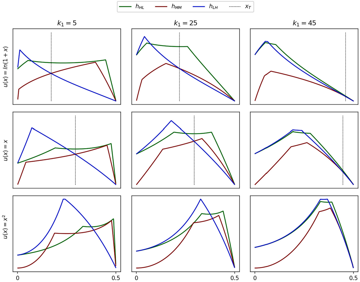
Fig. 7. The above plots depict the functions from which the stochastic potentials of the conventions can be computed by taking the ceiling. The plots are drawn, from top to bottom, for u(x) = \ln(1+x) , u(x) = x , and u(x) = x^2 and, from left to right, k_1 = 5 , k_1 = 25 , and k_1 = 45 , while k_2 is kept fixed at 50. The threshold x_T , as it results from Proposition 1, is not identified for u(x) = x^2 , due to the strict convexity of the utility function.
