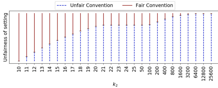
Fig. 5. k_1 is set at 10 while k_2 , which is represented in the x-axis, ranges from 10 to 25600. y-axis represents the unfairness of the setting, with minimum unfairness occurring when all possible splits are permitted, and maximum unfairness arising when only the fair split and the most extreme unfair splits are allowed. The red solid line indicates that the fair convention is stochastically stable; the blue dashed line indicated that an unfair convention is stochastically stable.
