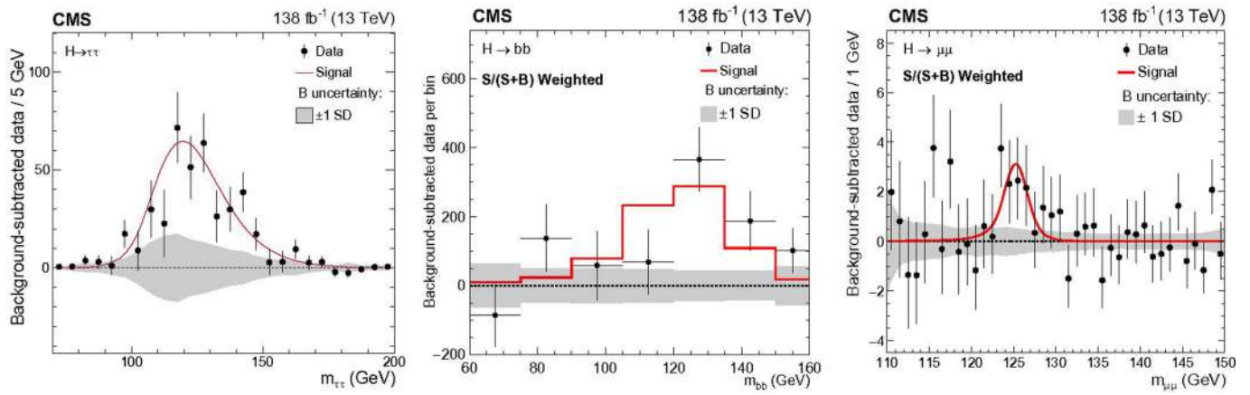
Extended Data Fig. 4 | Higgs boson mass peak in diferimion decay channels.
