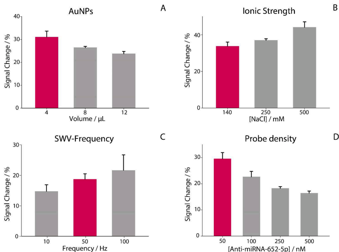
Fig. 1. A) Evaluation of AuNPs volume (4, 8, 12 \mu\text{L} ), B) Choice of NaCl concentration (140, 250, 500 mM), C) Optimization of the frequency of the square wave (10, 50, 100 Hz), D) Study of anti-miRNA-652 specific probe density (50, 100, 250, 500 nM). All the optimizations have been carried out in the presence of a target concentration of 40 nM.
