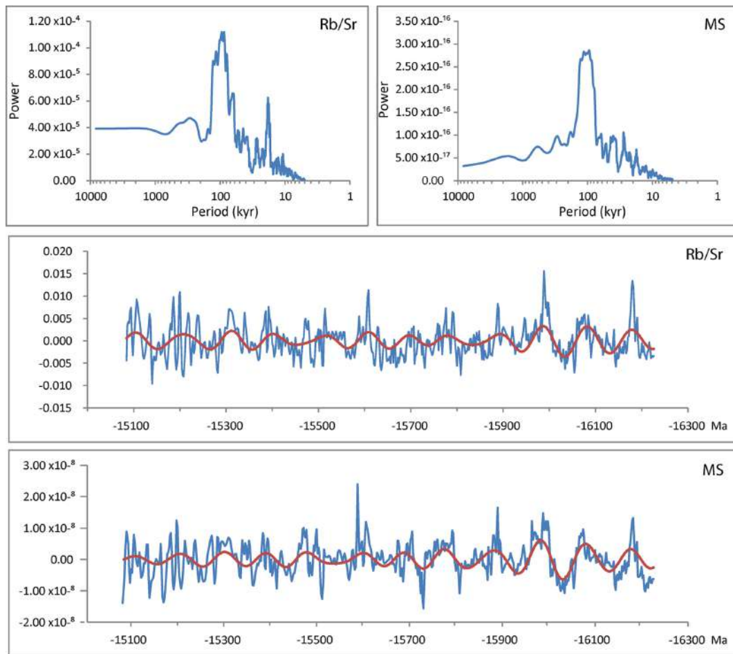
Figure 12. MTM spectra and results of bandpass filtering of the MS and Rb/Sr time series, based on the \sim 100 -kyr eccentricity tuned age model shown in Figure 11, showing the dominance of the \sim 100 -kyr cycle in the section (from Turco et al., 2017). The reader is referred to Turco et al. (2017) for similar spectra and results of filtering in the stratigraphic domain.
