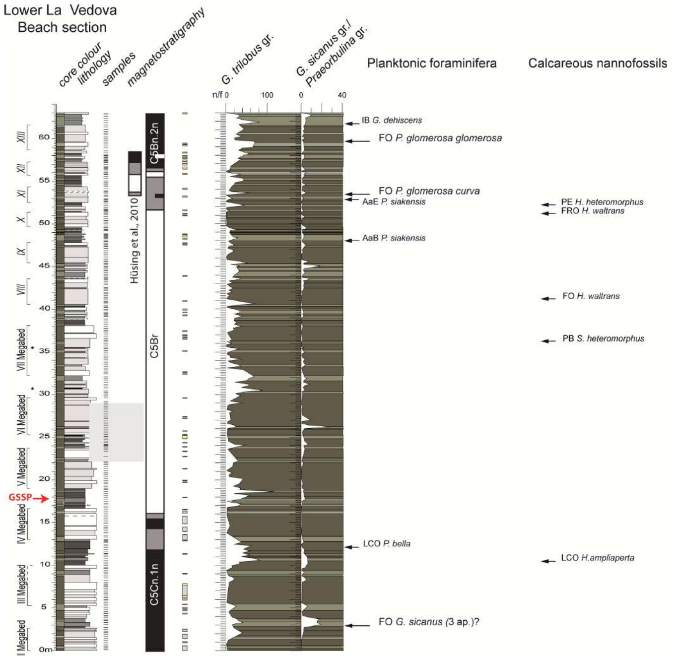
Figure 9. Globigerinoides trilobus gr. and G. sicanus-Praeorbulina gr. , and the position of bioevents linked to the G. sicanus-Praeorbulina lineage in the Lower La Vedova Beach section. The gray band indicates the missing interval in the composite section of Turco et al. (2011b). Gray boxes close to abundance curves indicate scarcity or very poor preservation of planktonic foraminifera. Bioevents acronyms: A a B (Acme a Beginning); A a E (Acme a End); FO (First Occurrence); FRO (First Regular Occurrence); Ia1, Ia2 (abundance Influx); IB (Influx Beginning); LCO (Last Common Occurrence); PB (Paracme Beginning); PE (Paracme End). The pattern in Globigerinoides trilobus gr. follows the larger-scale cyclicity in the section and to lesser extent the smaller-scale cyclicity represented by the greenish marl layers. The red arrow indicates the proposed GSSP level (modified after Turco et al., 2017).
