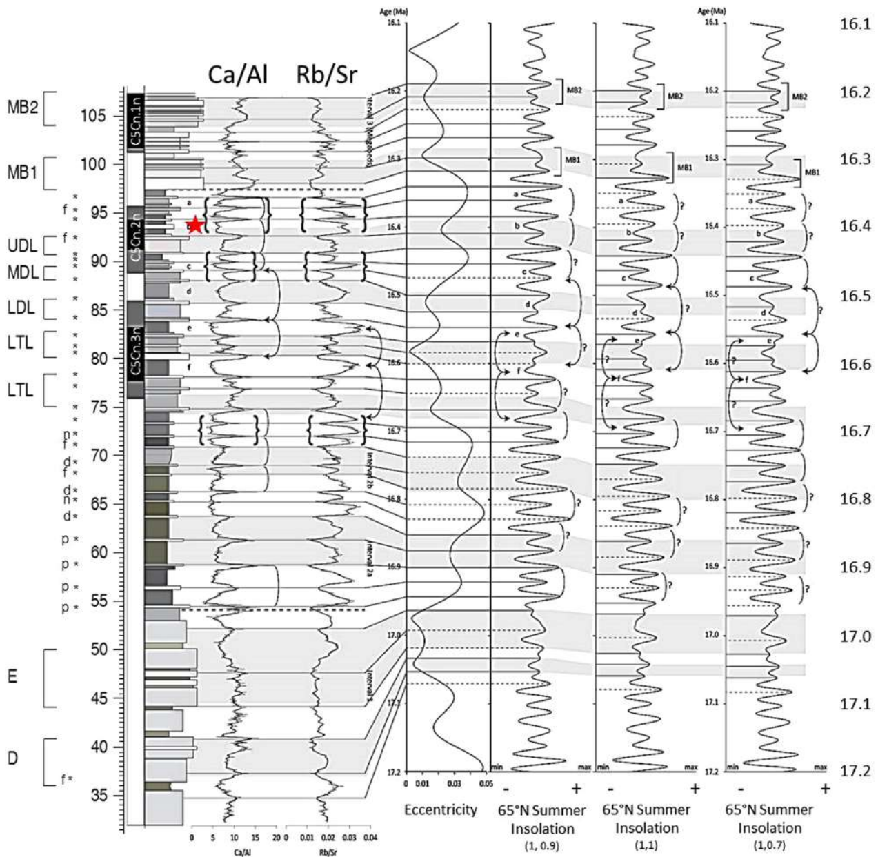
Figure 15. Magnetostratigraphy and astronomical tuning of the Monte Cardeto section. Ca/Al and Rb/Sr records have been tuned to the eccentricity and 65°N summer insolation curves. Red star marks the P. siakensis acme associated with subchron C5Cn.2n (van Peer, 2013; Turco et al., 2019).
