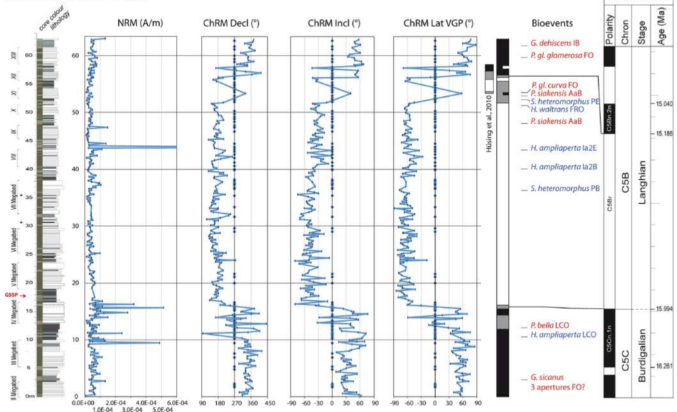
Figure 10. ChRM declination, inclination, VGP latitude, position of calcareous plankton events and correlations of the Lower La Vedova Beach section to the ATNTS2020 (Raffi et al. 2012). Bioevent acronyms: A_aB ( Acme a Beginning ); A_aE ( Acme a End ); FO ( First Occurrence ); FRO ( First Regular Occurrence ); Ia1, Ia2 ( abundance Influx ); IB ( Influx Beginning ); LCO ( Last Common Occurrence ); PB ( Paracme Beginning ); PE ( Paracme End ). Planktonic foraminiferal and calcareous nannofossil events are indicated in red and blue respectively. The red arrow indicates the proposed GSSP level (modified after Turco et al., 2011b, 2017).
