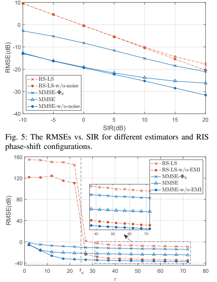
Fig. 6: The RMSEs vs. \tau for different estimators and RIS phase-shift configurations.
