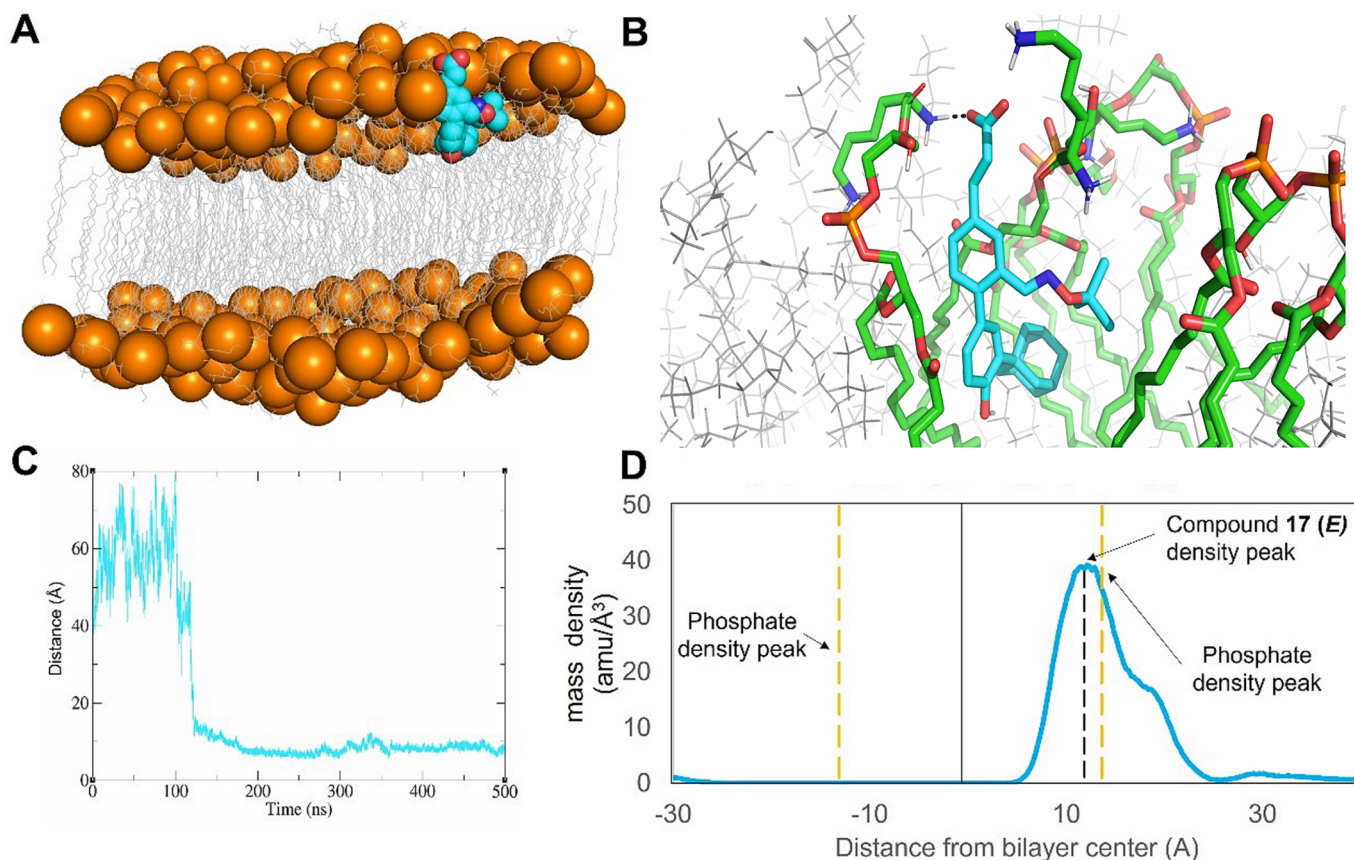
Fig. 4. A: Representative snapshot extracted from MD trajectories (500 ns – the representative frame of the most populated cluster is shown) describing the membrane/17( E ) interaction. The ligand is shown as cyan spheres, while phospholipids are represented as grey lines, with their phosphorous atoms highlighted as orange spheres; B: magnification of the interaction between 17( E ) (cyan sticks) with the membrane residues within 5 Å from the compound (shown as green sticks), the polar interaction is highlighted by a black dashed line; C: plot of the distance between 17( E ) and its binding site on the S. aureus membrane along MD trajectories; D: mass density profile of 17( E ) with the corresponding peak highlighted by black dash line. The density peaks of the lipid phosphate groups are indicated with orange dashed lines. Maximums of mass density in membrane are at -13.125 Å and 13.625 Å. (For interpretation of the references to colour in this figure legend, the reader is referred to the web version of this article.)
