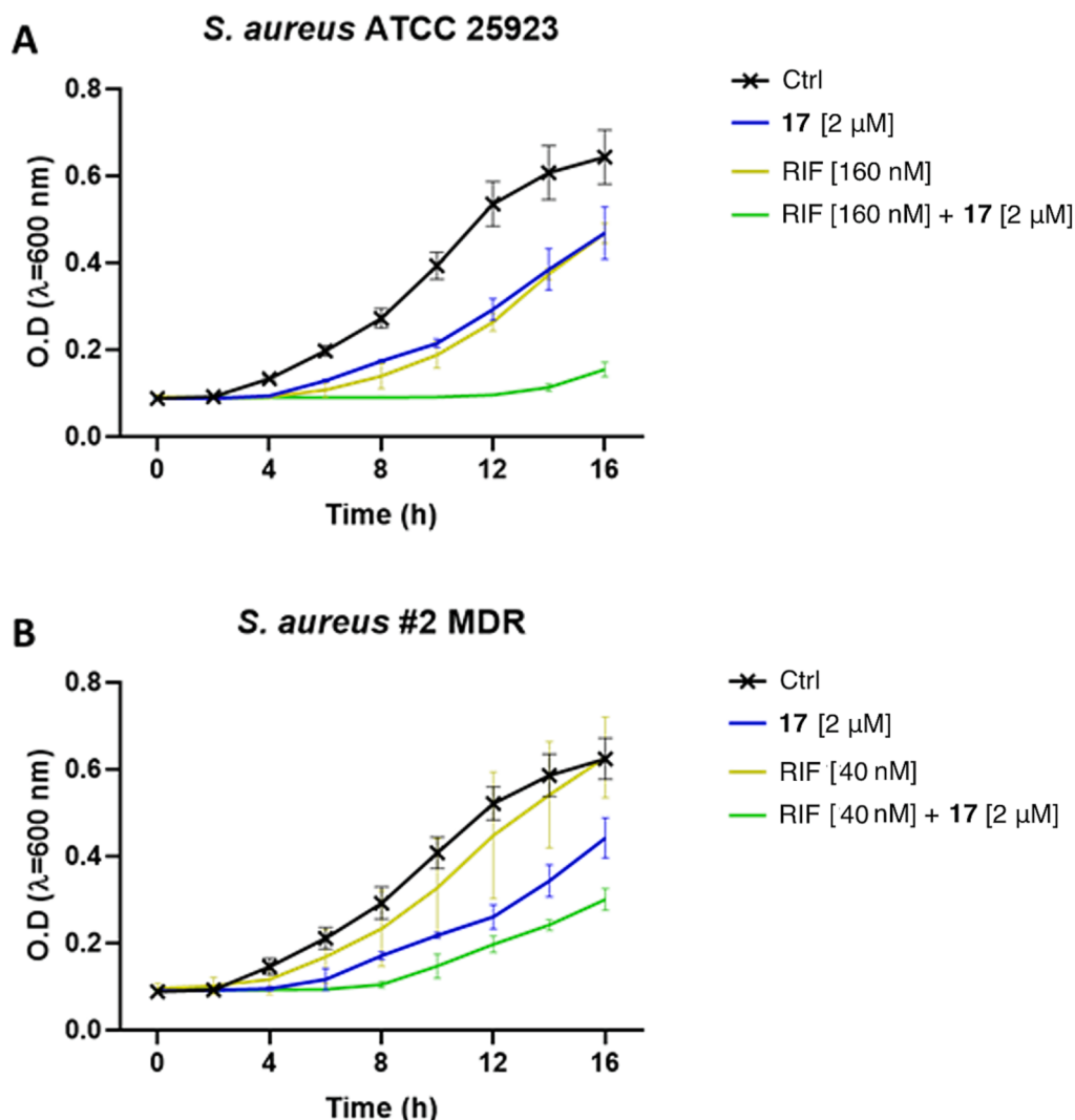
Fig. 9. Growth kinetics of (A) S. aureus ATCC 25923 and (B) S. aureus #2 MDR strains in the presence of rifaximin (RIF) at 1/2 MIC (yellow lines) in presence of compound 17 at its 1/2 MIC (2 \mu M, blue lines) as well as in the presence of their combinations (green lines). Results are the mean \pm standard deviation (SD) of three independent experiments. (For interpretation of the references to colour in this figure legend, the reader is referred to the web version of this article.)
