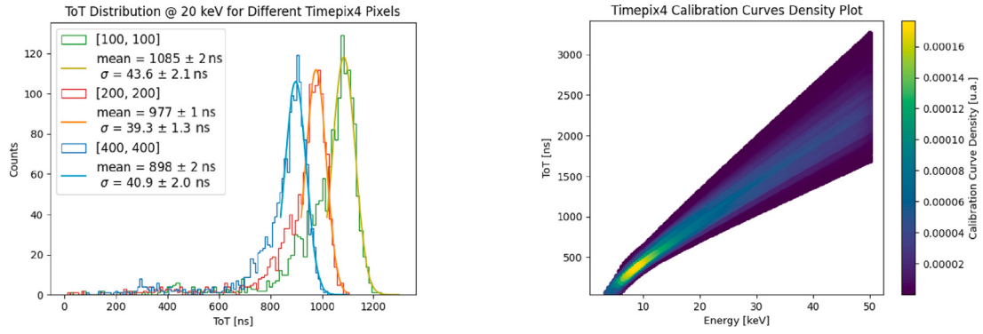
Fig. 3. Left: ToT distribution measured by three pixels at 20 keV (pixel coordinates are reported in the legend); the Gaussian fit on each ToT distribution is also reported (results in the legend), highlighting the asymmetric interval. Right: density plot of the calibration curves for all the Timepix4 pixels.
