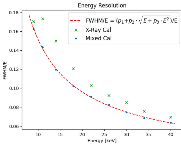
Fig. 8. Timepix4 energy resolution obtained with the X-ray calibration procedure (green) and with the mixed calibration procedure (blue). The Gaussian broadening energy function is superimposed to the mixed calibration data. The obtained fit parameters and the \chi^2 are: p_1 = 0.59 keV, p_2 = 0.29 keV 1/2 , p_3 = 3.15 \cdot 10^{-3} keV -1 , \chi^2_{\text{reduced}} = 0.63 , \chi^2_{\text{reduced}} = 0.79 .
