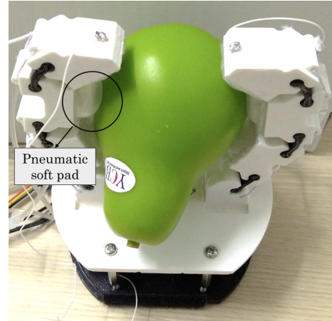
Fig. 1: Grasp performed by the SoftPad Gripper, a tendon-driven gripper equipped with pneumatic pressure sensors.
