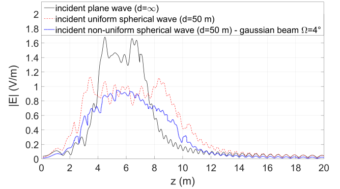
Fig. 7. Comparison of the reradiated field predicted with the ray model along the dashed green line in Fig. 5 in 3 different cases: a) incident plane wave (black line), b) incident uniform spherical wave (red dashed line), c) incident non-uniform spherical wave with gaussian profile and divergence \Omega = 4^\circ (blue dotted line)
