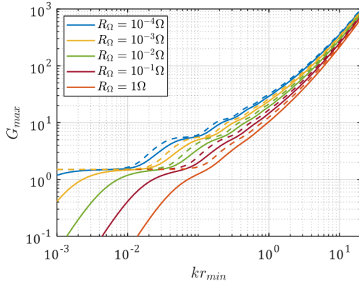
Fig. 3. Continuous lines: maximum gain of non-resonant (externally tuned) antennas calculated for different values of R_\Omega as a function of kr_{min} . Dashed lines: corresponding directivity obtained by G_{max}/\eta .
