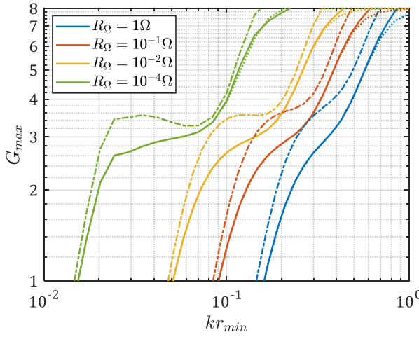
Fig. 10 Maximum gain of self-resonant antennas calculated for different values of R_\Omega (in Ohm) as a function of kr_{min} using the full series in (16) (continuous lines). Dotted lines: first two terms of the series in (16). Dash-dotted lines: directivities obtained by G_{max}/\eta with the full series.
