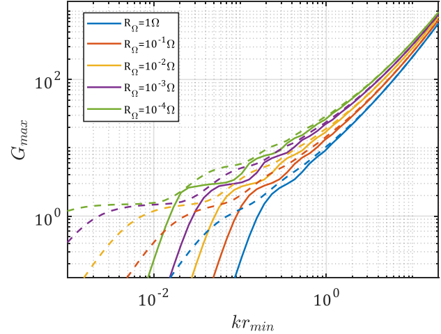
Fig. 5 Maximum antennas gain calculated for different values of R_0 as a function of kr_{min} . Dashed lines: externally tuned antennas. Continuous lines: self-resonant antennas.
