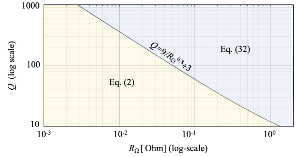
Fig. 12 Region of validity of the formulas for Q -bounded maximum gain with losses (eq. 32) and without losses (eq. 2). For Q < 9 / R_\Omega^{0.8} + 3 eq. (2) can be used with a maximum error less than 7% for all antenna sizes.
