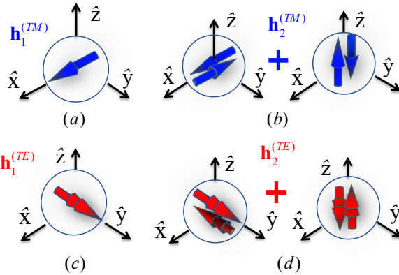
Fig. 8. Elementary sources associated with the far field pattern of dipolar \mathbf{h}_1^{(TM)} (a), \mathbf{h}_1^{(TE)} (c) and quadrupolar \mathbf{h}_2^{(TM)} (b) \mathbf{h}_2^{(TE)} , (d) contributions. Electric dipoles (TM) are denoted in blue with a single arrow and magnetic dipoles (TE) in red with a double arrow. The vertical doublet is aligned along x for electrical dipoles and along y for magnetic dipoles.
