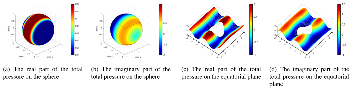
Fig. 5. Rigid scattering of a plane wave on a sphere with \kappa = 2 : on and off surface total pressure distributions.
