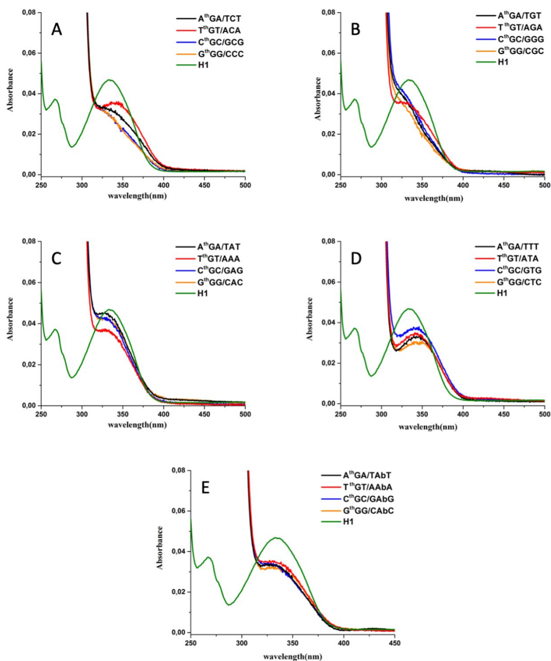
Figure 2: Absorption spectra of th G-labelled matched (A) and mismatched (B-E) (+)/(-)PBS duplexes. In the mismatched duplexes, th G was opposite G (B), A (C), T (D) or an abasic site (E). In each panel, the neighboring residues of th G were systematically varied. The concentration of all duplexes was 10 μM. The absorption spectrum of the H1 tautomer of free th G at the same concentration in water is included for comparison (green spectra). All experiments were done in 25 mM TRIS-HCl buffer (pH=7.5), 30 mM NaCl and 0.2 mM MgCl 2 .
