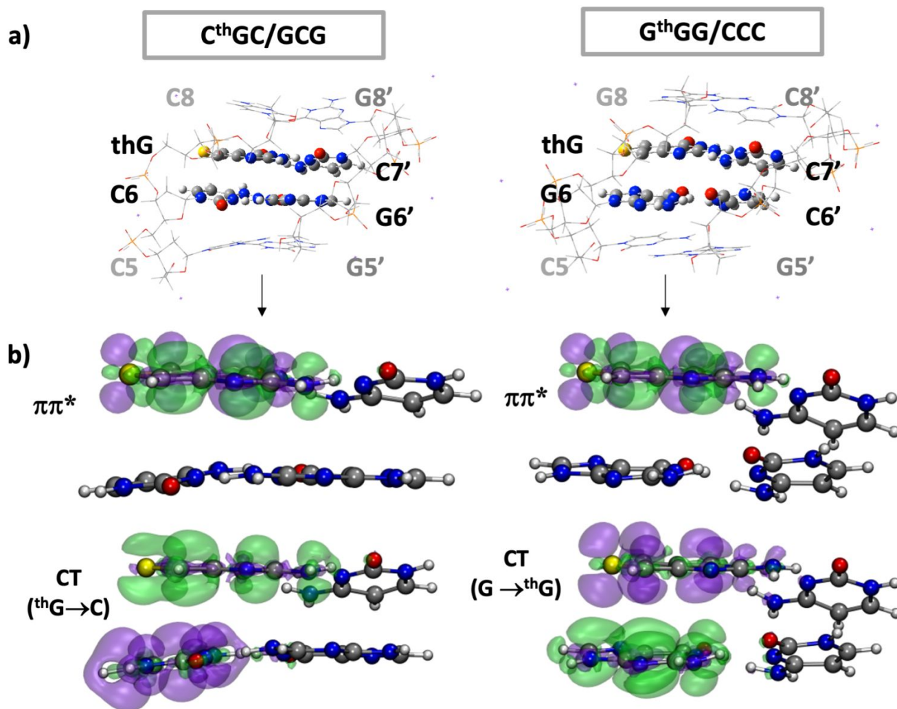
Figure 5: Ground-state geometries (A) and excited-state electronic densities (B) of the matched duplexes. A) Most relevant geometries for the optimized minima at the QM(PCM/M052X/6-31G(d))/MM level of theory. Nucleobases treated at the QM level are in ball and sticks, whereas the MM system is depicted in lines. Numbering of residues is as in Figure 1. B) Excited-state density difference ( S_n-S_0 ), green means negative difference (i.e from where the electron moves) while purple indicates more density (i.e where the electron moves to).
