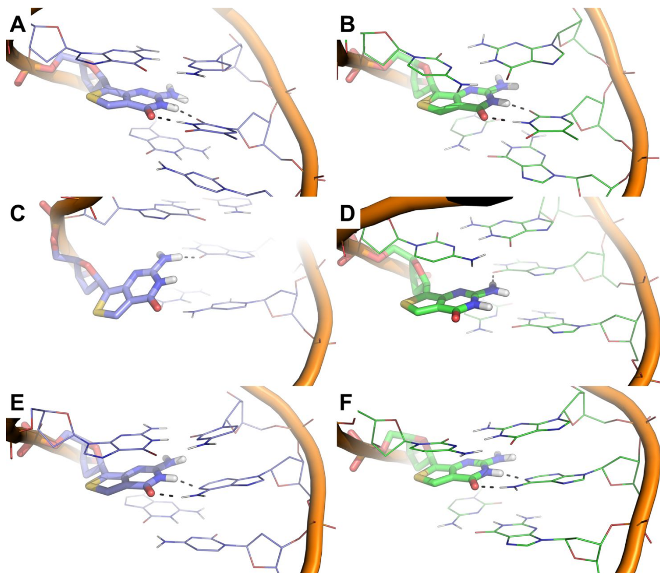
Figure 6. Conformational analysis of mismatched (+)/(-)PBS duplexes where th G is flanked by G and C bases. A) Magnification of the interaction of the th G-T base pair with flanking G residues in the G th GG/CTC duplex. B) Magnification of the interaction of the th G-T base pair with flanking C residues in the C th GC/GTG duplex. C) Magnification of the interaction of the th G-G base pair with flanking G residues in the G th GG/CGC duplex. D) Magnification of the interaction of the th G-G base pair with flanking C residues in the C th GC/GGG duplex. E) Magnification of the interaction of the th G-A base pair with flanking G residues in the G th GG/CAC duplex. F) Magnification of the interaction of the th G-A base pair with flanking C residues in the C th GC/GAG duplex. th G is shown as sticks, other nucleotides are shown as lines while the phosphate backbone is shown as cartoon. H-bonds are shown as dashed lines. Mismatched duplexes where th G is flanked by G are coloured blue, while systems bearing th G flanked by C are coloured green.
