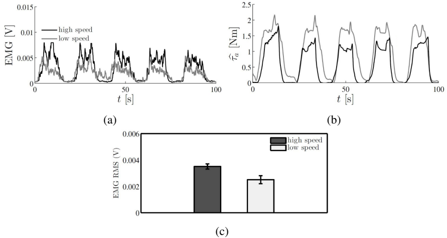
Figure 1.8: Evaluation of the effectiveness of the assistance modulation at different elbow speeds. (a) The amplitude of the EMG activities are shown when a single subject performed the elbow motions at two different velocities. When the subject moves slower (b) The assistive torques at a lower (light grey) and higher (dark grey) elbow speed motion. (c) Comparison of the EMG activity at low and high speed of movement with the proposed controller.
