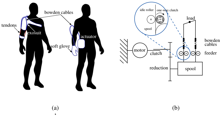
Figure 1.1: Components of the exosuits (a) and schematics of the actuation units (b). (a) Both devices comprise a wearable component (exosuit or glove) and a proximally-located actuation unit that transmits power to the joints via bowden cables. (b) DC brushless motors drive a spool around which the artificial tendons are wrapped; an electromechanical clutch allows to couple and decouple the motor from the transmission, allowing the user to move freely on demand. A feeder mechanism, thoroughly described by In et al. [38], keeps the cables in tension around the spool.
