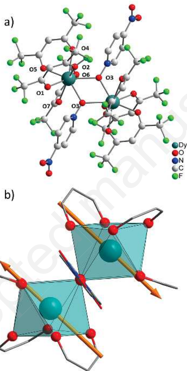
Fig. 1. a) Representation of the [\text{Dy}(\text{hfac})_2(\text{PyNO-NO}_2)_2] molecule (hydrogen atoms are omitted for clarity) b) Coordination environment of the Dy III ion with calculated easy magnetic axis as orange arrows. (For interpretation of the references to colour in this figure legend, the reader is referred to the web version of this article.)
