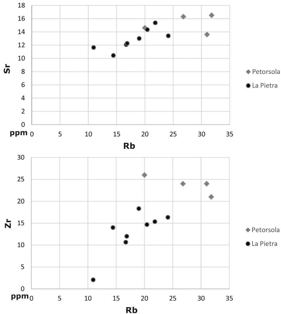
Figure 14. Scatter diagrams showing the values of Rb/Sr and Rb/Zr in radiolarite samples from the outcrops of La Pietra and Petorsola.
