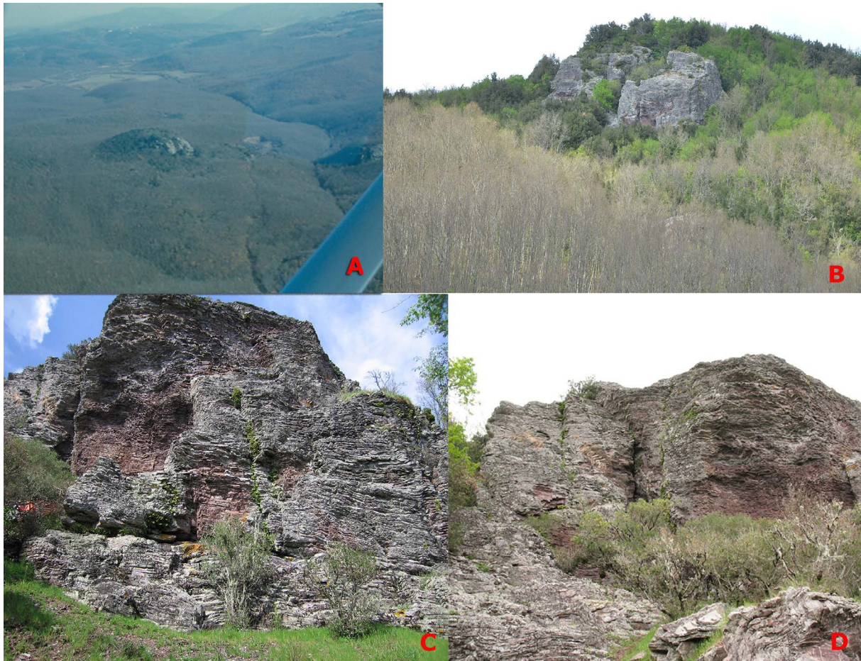
Figure 3. Different views of La Pietra rock cliff: A-air photograph with the Farma stream on the right; B-the outcrop seen from the opposite side of the Farma stream; C-detail of the south-eastern wall of the outcrop; D-detail of the southern wall of the outcrop.
