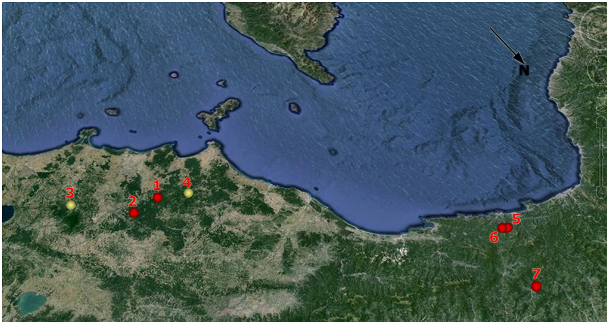
Figure 2. Location of the radiolarite exploitation sites mentioned in the text. 1-La Pietra quarry and workshop; 2-Albatreri quarry and workshop; 3-Petorsola workshop; 4-Poggio Mutti workshop; 5-Valle Lagorara quarry and workshop (Campana & Maggi 2002); 6-Serre di Liciorno quarry and workshop (Campana et al. 2013); 7-Ronco del Gatto quarry and workshop (Ghiretti 2003). (Satellite image: Google, Image Landsat 2015).
