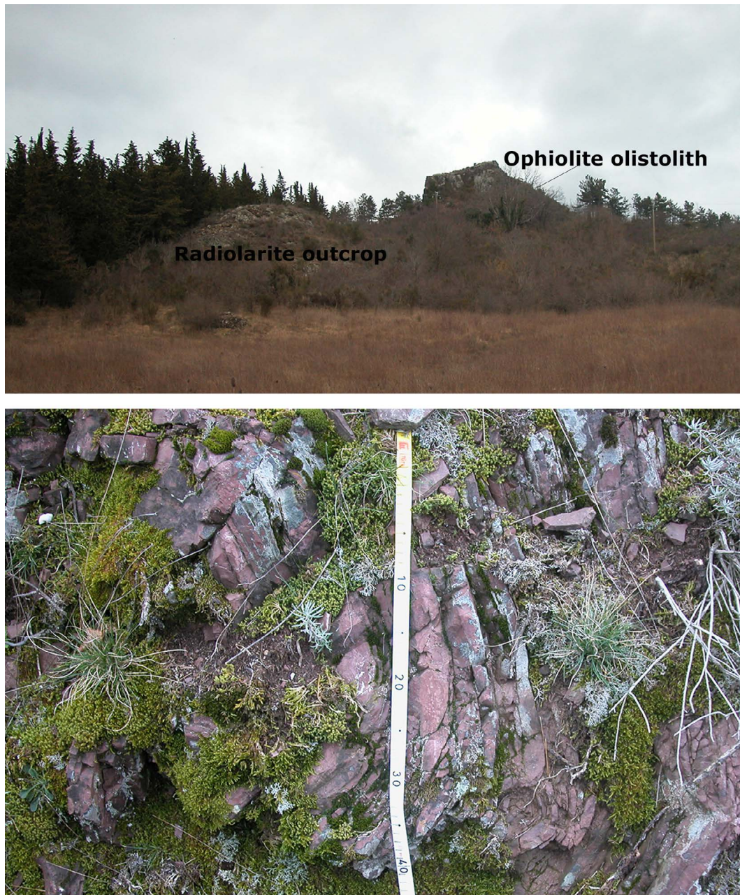
Figure 11. Petorsola ophiolite olistolith and radiolarite outcrop.
