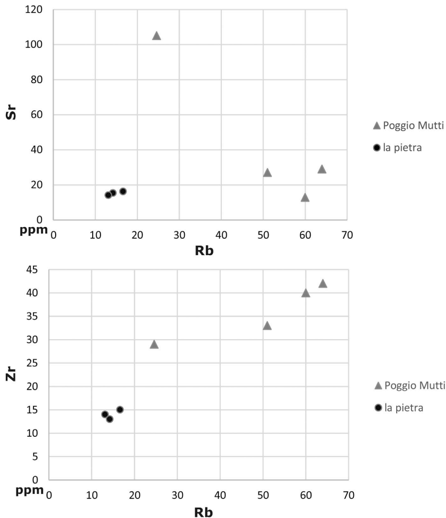
Figure 15. Scatter diagrams showing the values of Rb/Sr and Rb/Zr in radiolarite samples from the outcrops of La Pietra and Poggio Mutti.
