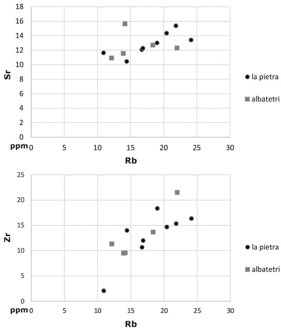
Figure 13. Scatter diagrams showing the values of Rb/Sr and Rb/Zr in radiolarite samples from the outcrops of La Pietra and Albatreti.
