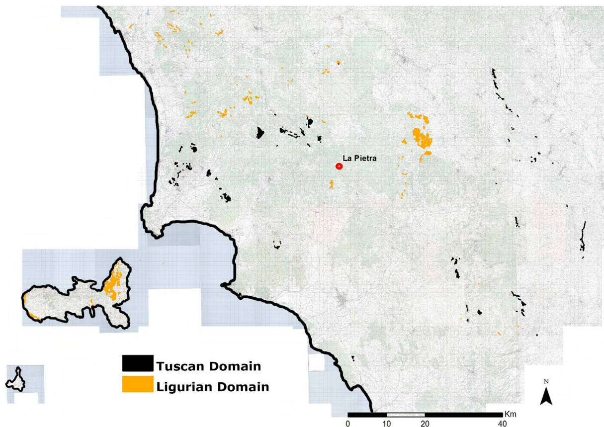
Figure 8. The radiolarite (“Diaspri”) outcrops of the Tuscan and Ligurian domains in the area of central-southern Tuscany with La Pietra. Map created with ArcGIS software. Data from Geodatabase of Tuscany (Regione Toscana 2015).
