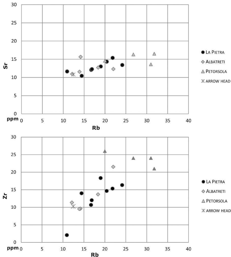
Figure 16. Scatter diagrams showing the elemental of Rb/Sr and Rb/Zr for the Copper Age radiolarite arrowhead of the Lanfredini collection against those of the La Pietra, Albatreti and Petorsola outcrops.
